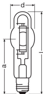
HQI-BT 400 W/D PRO
